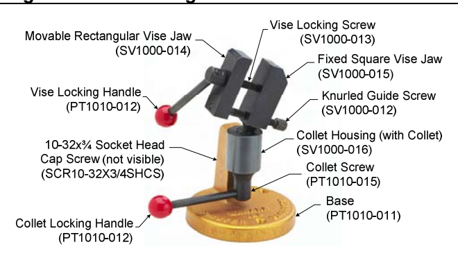
Figure 2. Swiv-O-Ling Vise Assembled
