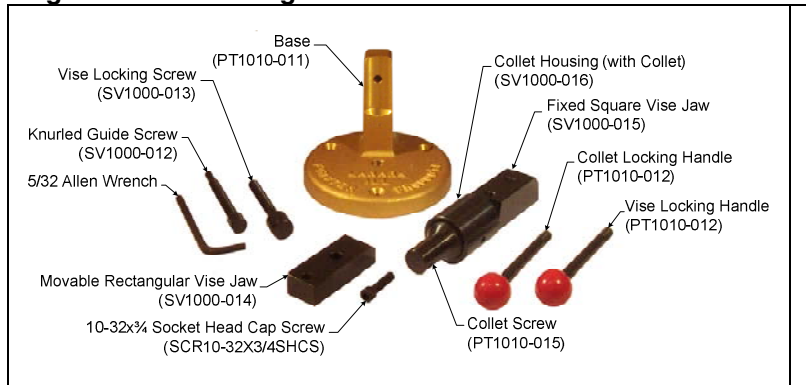
Figure 1. Swiv-O-Ling Vise Unassembled
