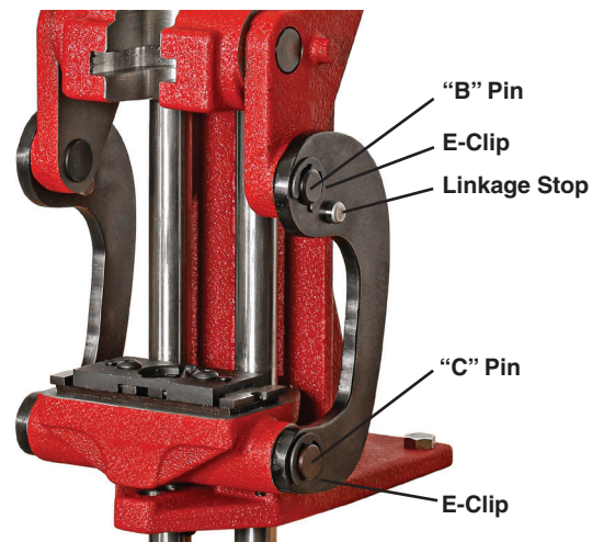
Figure 2. Curved Links
