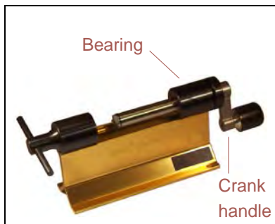
Figure 2. Crank Handle Assembly
