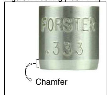
Figure 2. Bushing (Bush-XXX)
