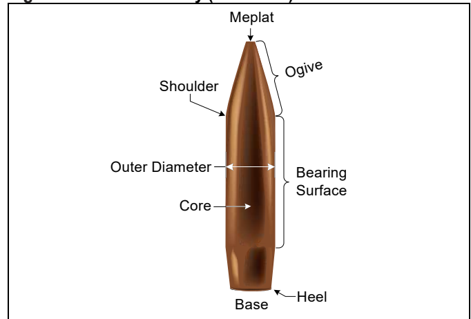
Figure 2. Bullet Anatomy (Flat Nose)
